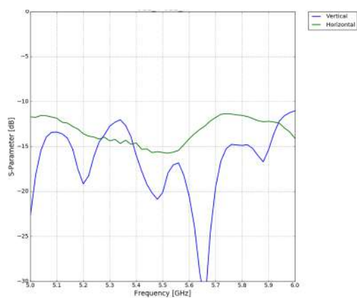
Return Loss
